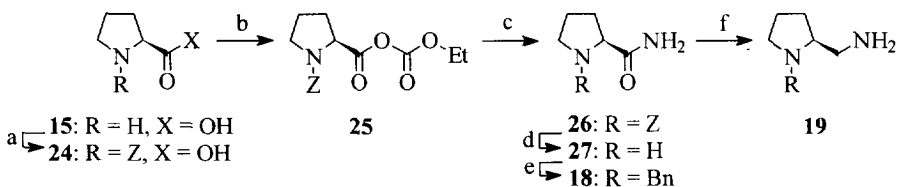
Scheme 5. a. \text{PhCH}_2\text{OCOCl} ( \text{ZCl} ), \text{NaOH} , \text{H}_2\text{O} , 92 %; b. N -methylmorpholine, \text{ClCO}_2\text{Et} , \text{CH}_2\text{Cl}_2 ; c. \text{NH}_3 , \text{CH}_2\text{Cl}_2 , -25^\circ\text{C} , total of 2 steps: 92 %; d. \text{Pd/C} , \text{H}_2 , \text{MeOH} , 83 %; e. \text{BnBr} , \text{CH}_2\text{Cl}_2/\text{MeOH} 4/1, 70 %; f. \text{Li}[\text{AlH}_4] , \text{THF} , 81 %.
