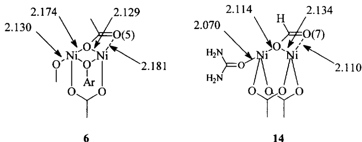
Figure 3. Core of complex 6 and 14 . 23c (bond distances in Å, other ligands omitted for clarity)
