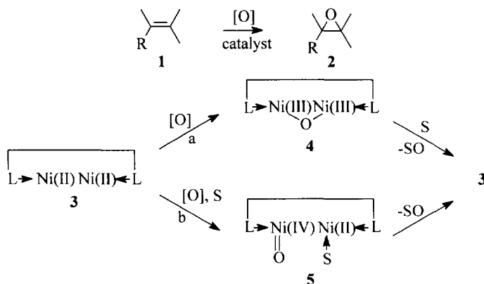
Scheme 1. Bimetallic shunt or rebound mechanism in catalytic epoxidation. (S = substrate, [O] = single oxygen donor).
