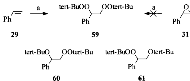
Scheme 11. a. tert -butyl hydroperoxide, 1.5 mol% 7 , \text{CH}_2\text{Cl}_2/\text{NaOH}/\text{H}_2\text{O} , 25 %.
