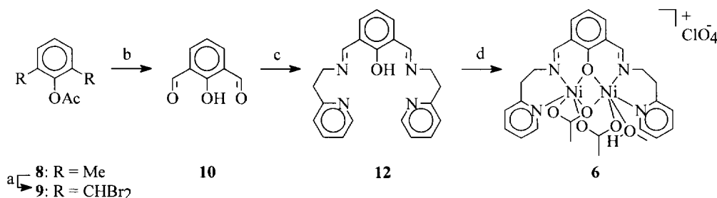
Scheme 2. a. hν , Br 2 , CCl 4 , 64 %; b. KOH/H 2 O Δ, 73 % c. 2-pyridin-2-yl-ethylamine ( 11 ), MeOH, Δ, 100 % d. Ni(OAc) 2 ·4H 2 O, Na(ClO 4 )·H 2 O, MeOH, Δ, 67 %.
